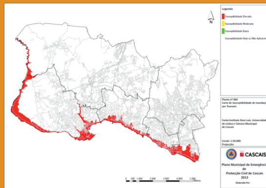
Flood susceptibility map caused by a tsunami
