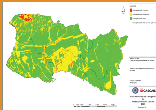
Seismic soil susceptibility map
